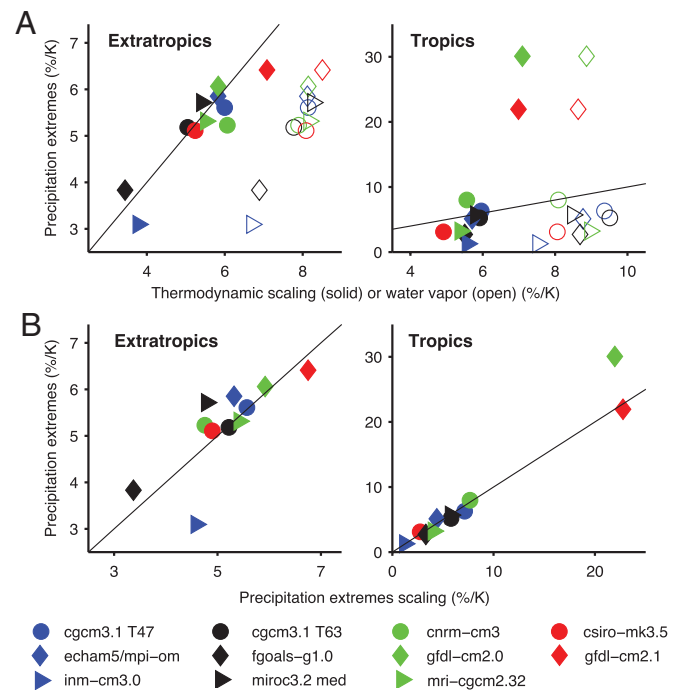
Fig. 3. Fractional changes in the 99.9th percentile of daily precipitation for each model versus changes in atmospheric water vapor content and scalings for precipitation extremes. (A) Atmospheric water vapor content (open symbols) and the thermodynamic scaling that neglects changes in upward velocity (solid symbols). (B) Full scaling for precipitation extremes. The fractional change are relative to 20th-century values, averaged over the extratropics (Left) or tropics (Right) and normalized by the change in surface air temperature averaged over the extratropics or tropics. Solid lines correspond to one-to-one relationships. The extratropics are defined as the regions poleward of 30° latitude, and the tropics are defined as the region equatorward of 30° latitude.
